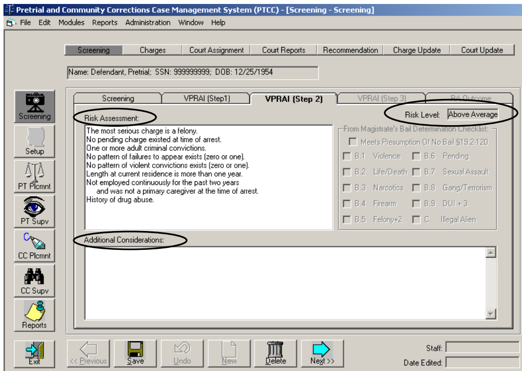
Figure 10. VPRAI (Step 2) Tab in Screening Module
